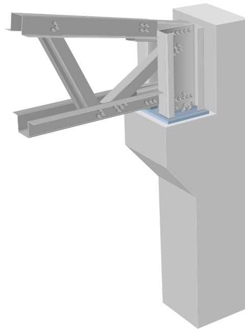
HINGED CONNECTION TO REINFORCED CONCRETE COLUMN
